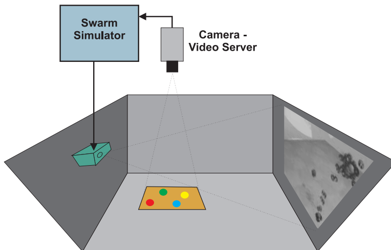
Figure 1: Schematic diagram of SwarmArt 2002. The system projects images of a simulated swarm onto a wall. The video server tracks the positions of coloured balls on a table. The positions of the balls set parameters for the swarm simulation, and change the behaviour of the entities in the projected image.
