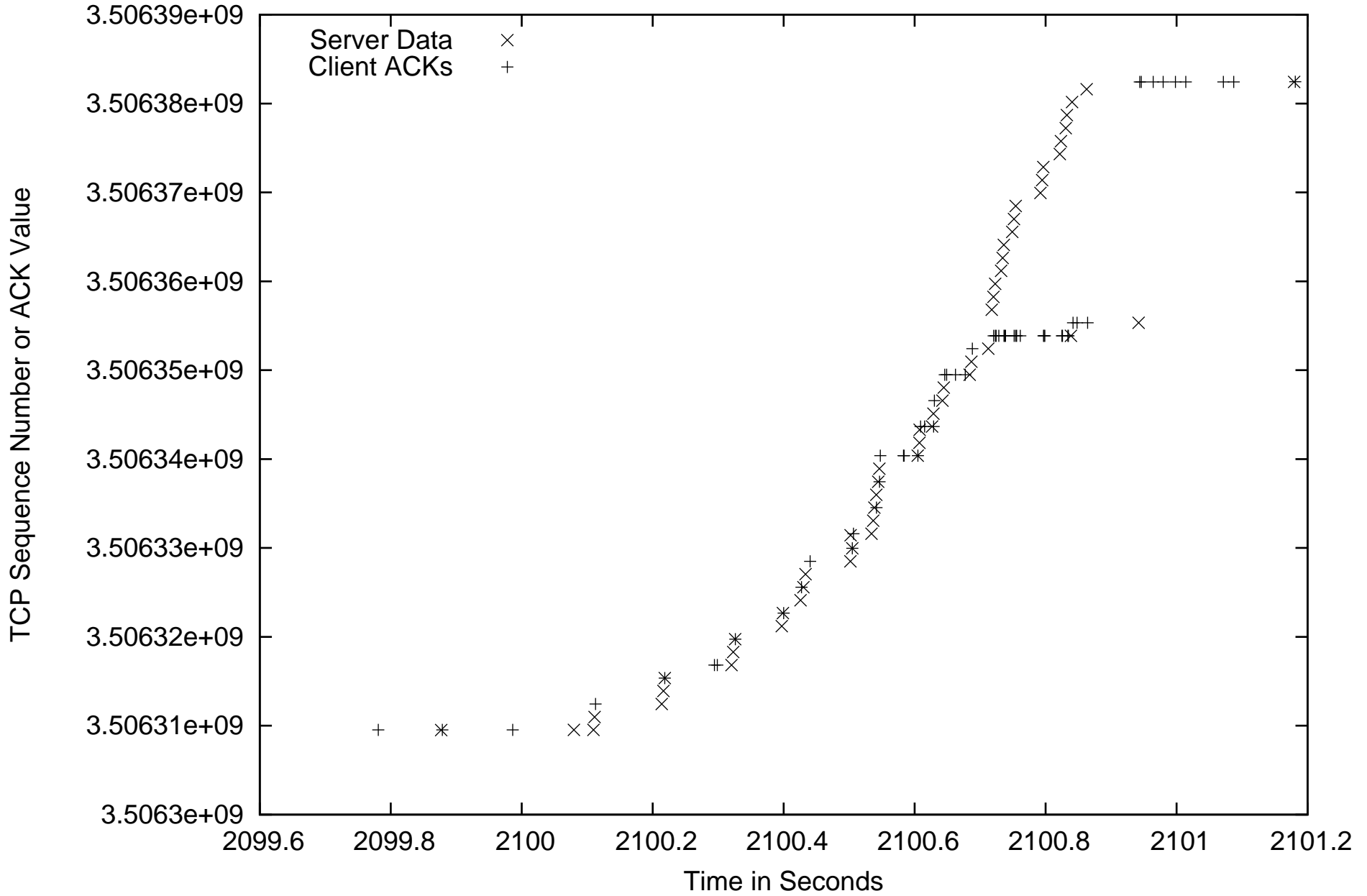
TCP Sequence Number Plot (206.16.0.188 port 1064)
