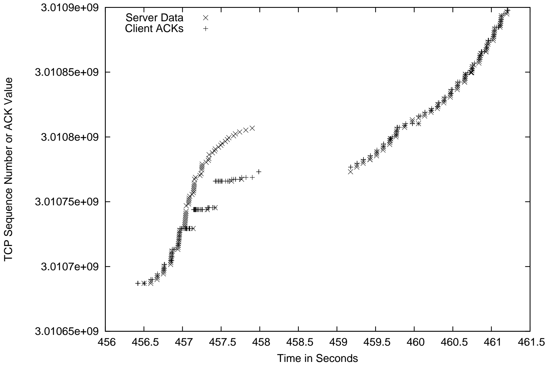
TCP Sequence Number Plot (64.143.96.175 port 1209)
