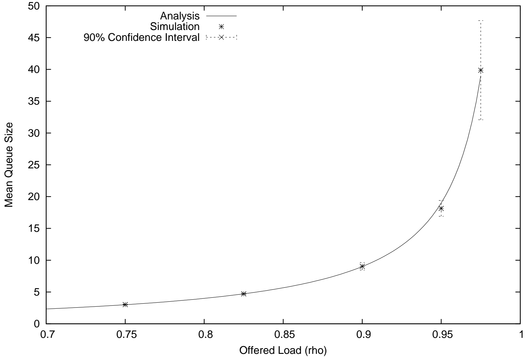
M/M/1 Validation Results: Mean Queue Size versus Load
