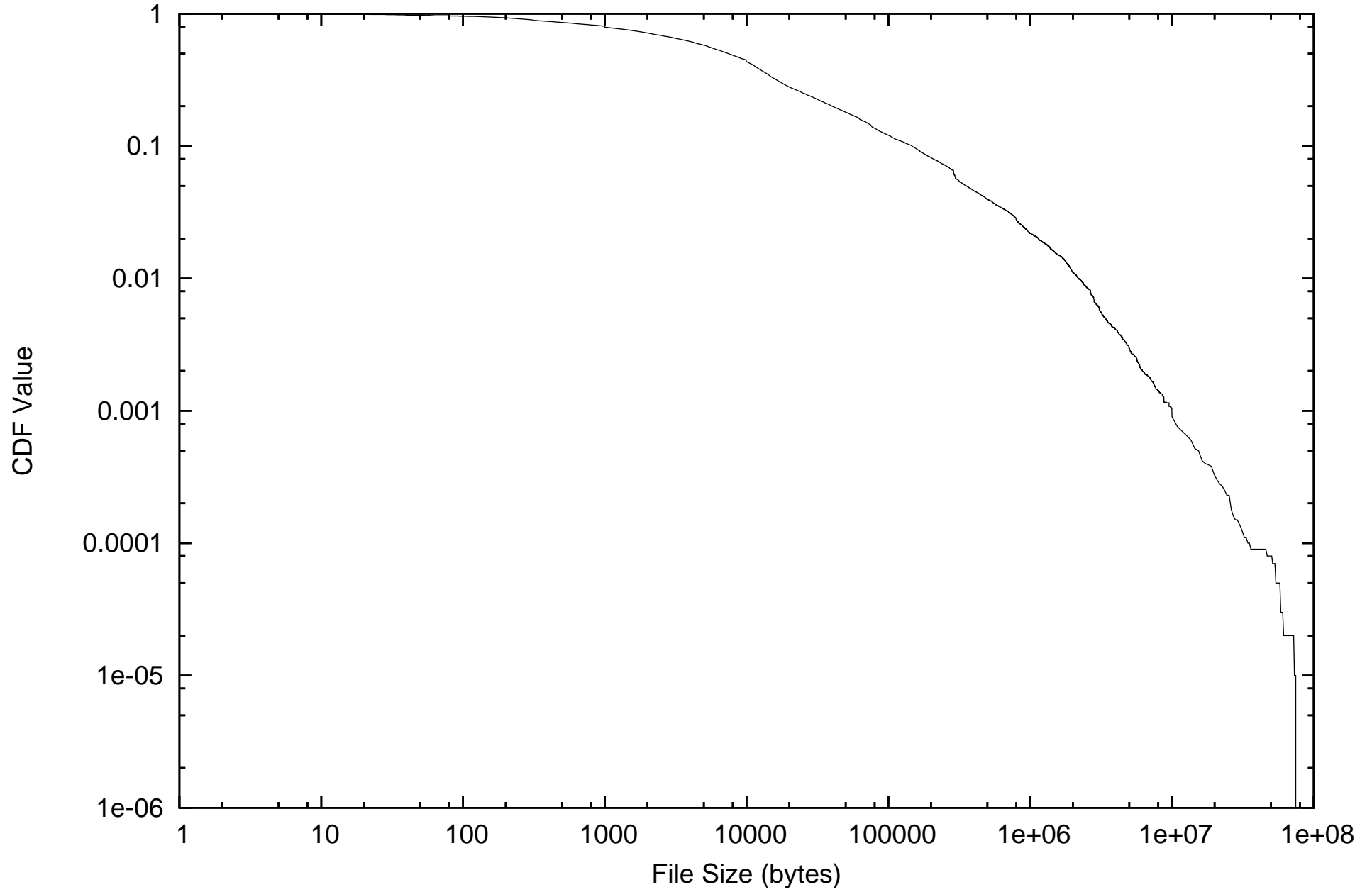
LLCD of File Size Distribution
