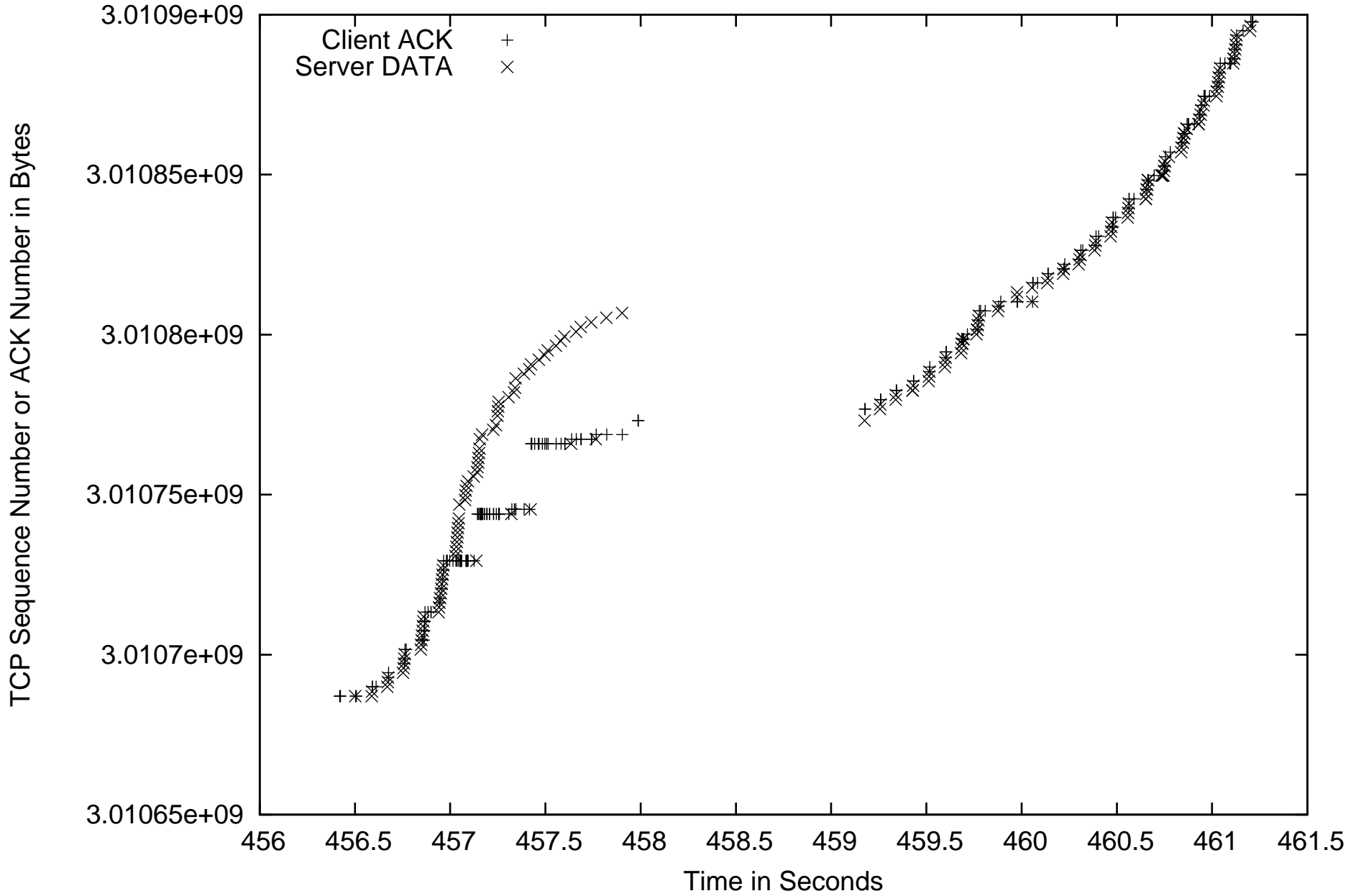
TCP Sequence Number Plot for TCP Connection (Port 1209)
