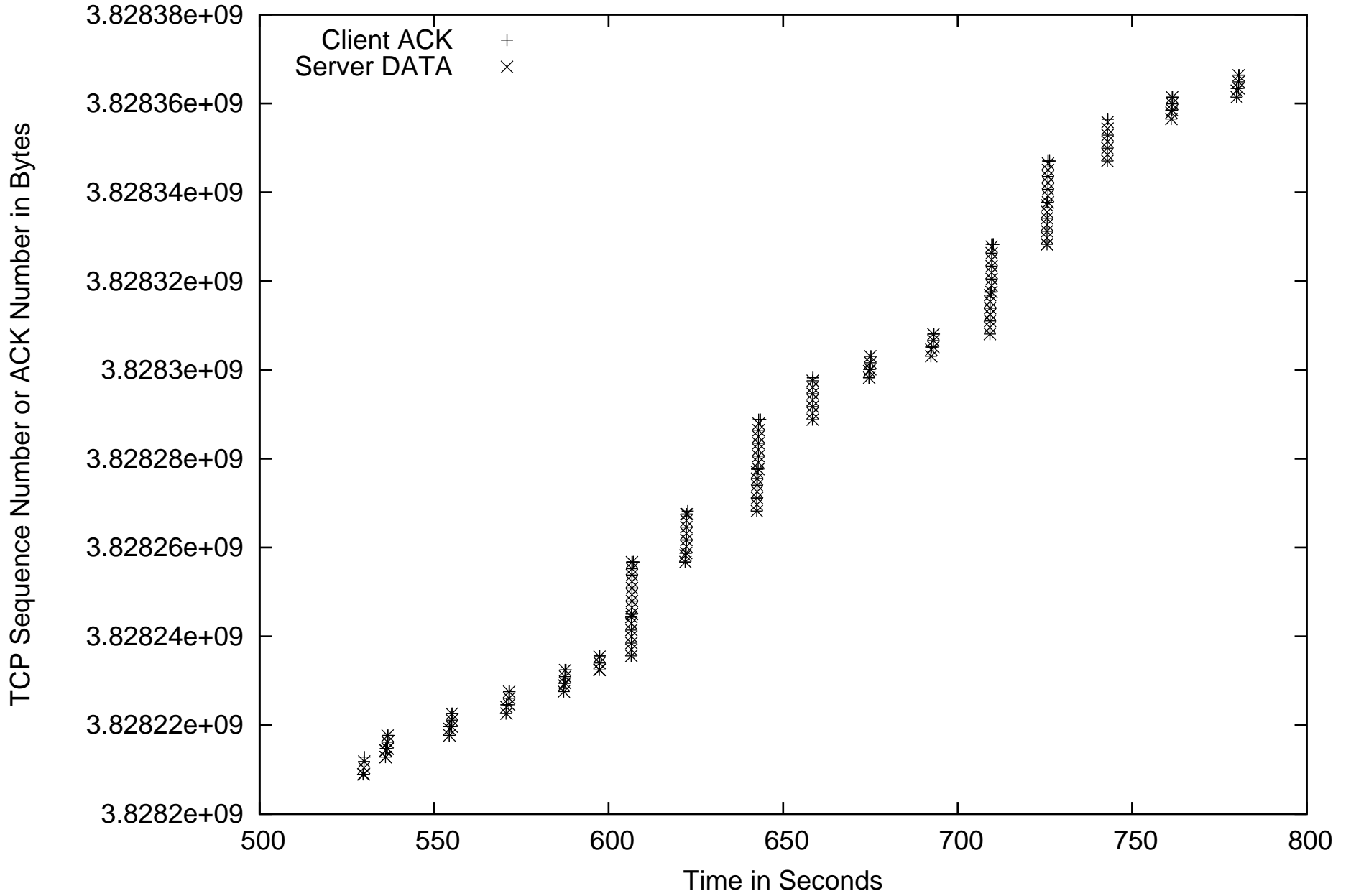
TCP Sequence Number Plot for TCP Connection (Port 1223)
