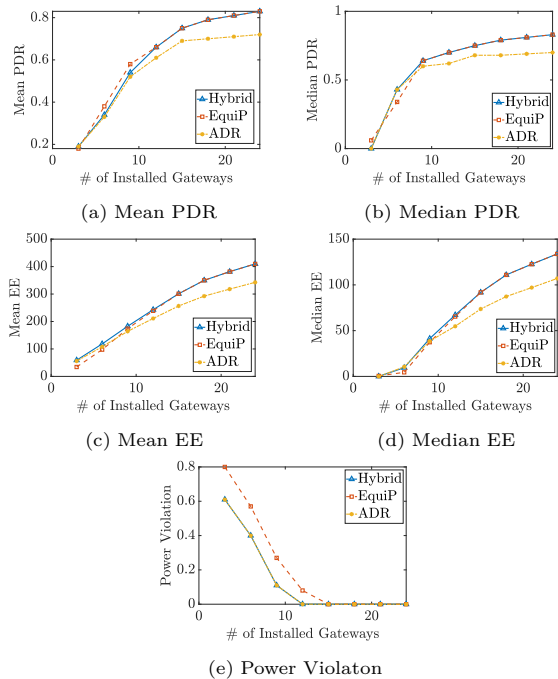
Fig. 7: Comparison of performance metrics achieved by different strategies with different number of installed gateways.
