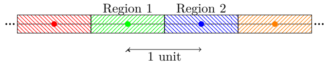
Fig. 3: Single-gateway access in the linear network. Each region indicates the set of EDs that communicate with the same gateway.
