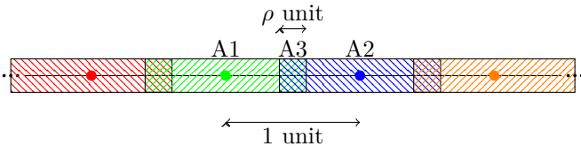
Fig. 4: Linear regular network with multiple-gateway access. The EDs in A1 and A2 are only heard by a single gateway, while EDs in A3 are heard by 2 gateways.
