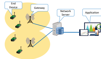
Fig. 1: A typical LoRa network architecture.
