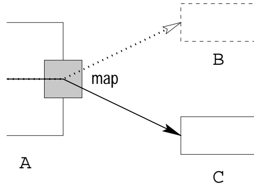
Fig. 3: An outgoing message is intercepted at the boundary of component A by a boundary map. The message contents can be manipulated and the message rerouted to a new recipient ( C ), all based on the previous history of the system. The originally intended recipient ( B ) need not be present in the system at all.
