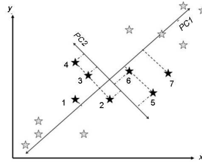
Figure 4: A geometrically-invariant vertex ordering is obtained by projecting onto the principal component axes (ascending order).
