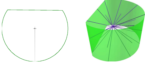
Fig. 13. The outline (left) and resulting projection surface (right) used to create the image shown in Figure 1.
