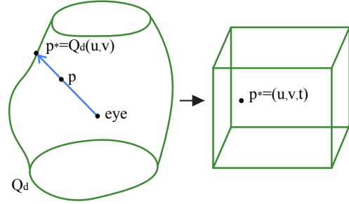
Fig. 10. When rasterizing we transform p from camera coordinates (x, y, z) to parameterized volume coordinates (u, v, t) . We can find (u, v) quickly by identifying the ray (with unique spherical coordinates) that passes through they eye, p , and p^* as shown on the left. On the right we produce interpret and rescale the volume parameters (u, v, t) as existing in the normalized device coordinate viewbox.
