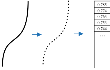
Fig. 11. Precalculation for outline and profile curves. The curve (left) is first sampled into point by arc-length (middle) and then the appropriate spherical coordinate ( \theta for outlines, \phi for profiles) is stored in an ordered array (right).
