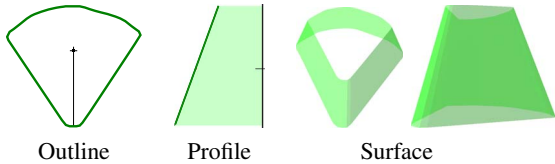
Fig. 7. An arc-length parameterized projection surface created with Equation 1. In outline diagrams the origin is marked; the descending line’s intersection with the outline indicates the seam. The front of the projection (the center of the image) is halfway along the arc-length of the entire outline from the seam. Profile diagrams show the profile as well as a light fill to relate the curve to the up axis.
