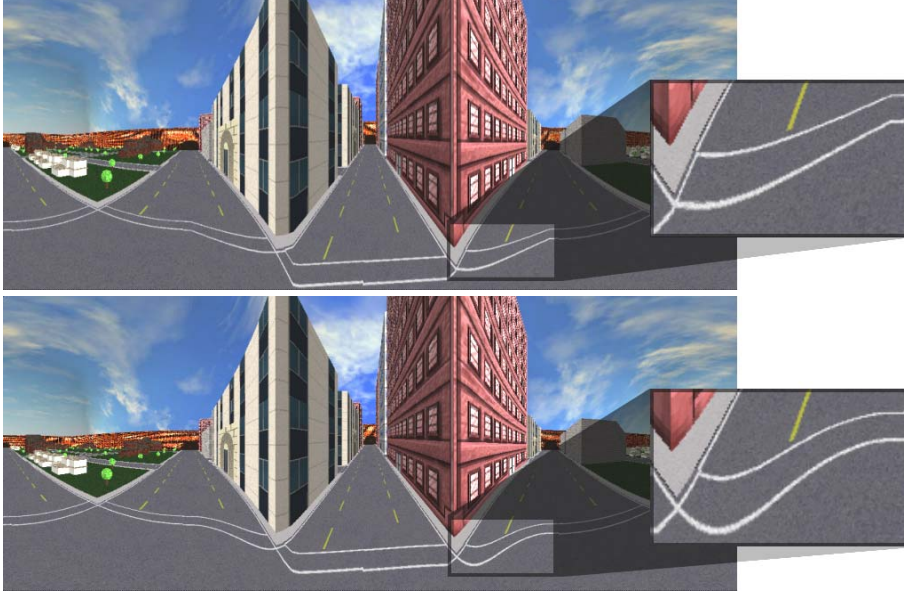
Fig. 9. Comparison between linear (top) and Bézier based (bottom) interpolation between profiles. Transitions between profiles are most noticeable in the magnified area examining the crosswalk lines. With linear interpolation the crosswalk lines transition sharply; Bézier interpolation creates a curved transition.
