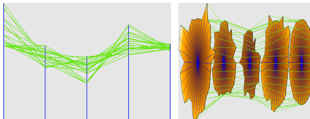
(a) Data items selected with help of color scale. (b) Unfolded selected set of data items.
