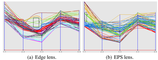
Figure 15: Lens interaction with Parallel Coordinates.
