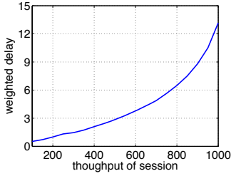
Fig. 2. Weighted delay for a single session as the throughput of the session is increased.
