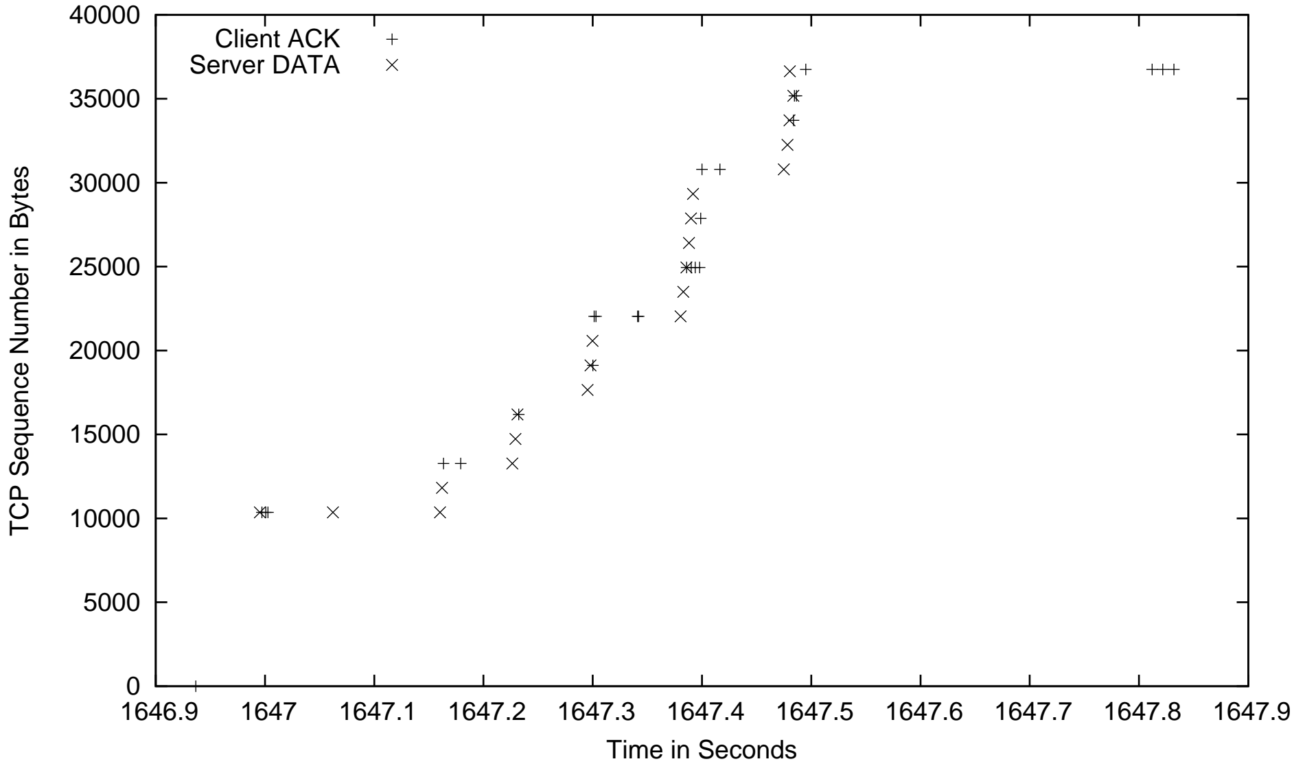
TCP Sequence Number Plot for TCP Connection (Port 1064a)
