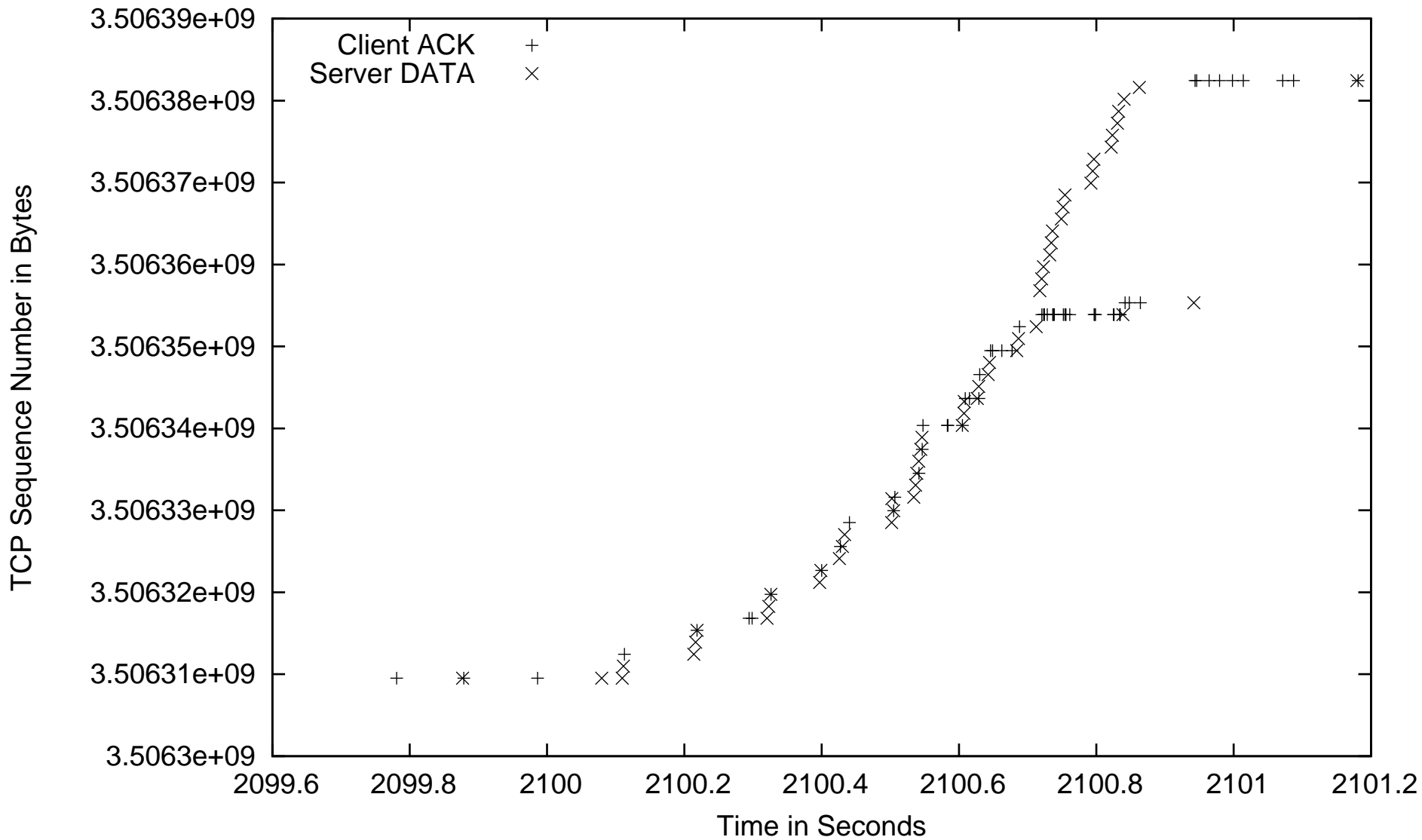
TCP Sequence Number Plot for TCP Connection (Port 1064b)
